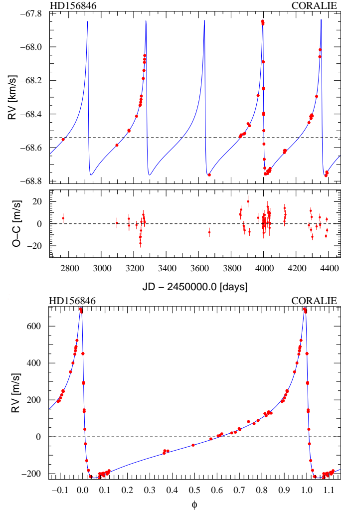
Fig. 2. Same as Fig. 1 for HD 156846.
