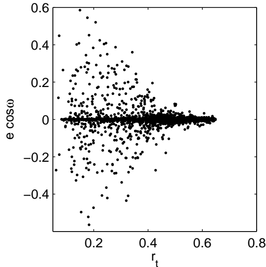
Figure 11. e \cos \omega vs. the total radius
