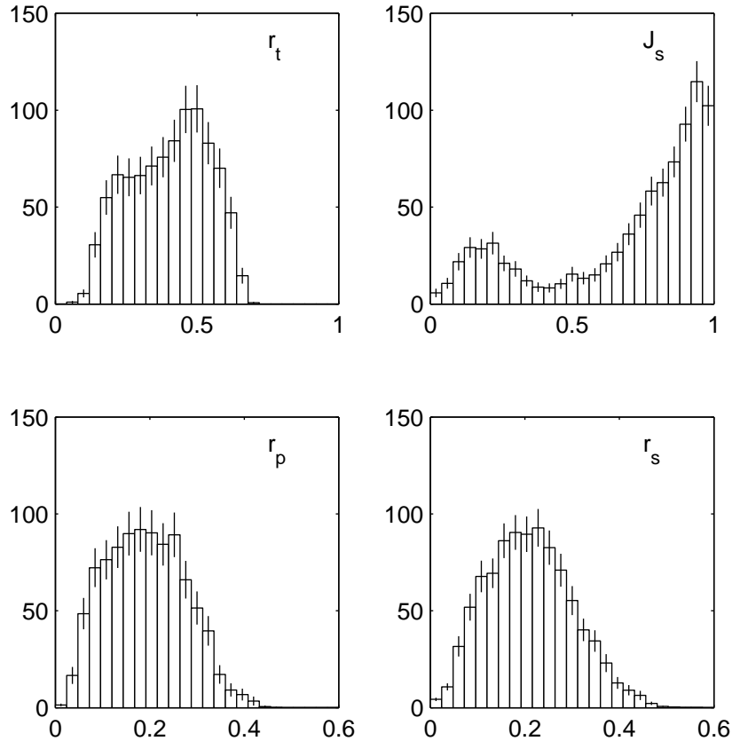
Figure 6. Histogram of the derived elements.
