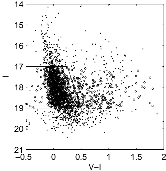
Figure 5. The I -magnitude as a function of the averaged V - I colour. Binaries excluded from the trimmed sample by the previous constraints are represented by dots. All 1131 binaries still in the trimmed sample are presented by small circles.
