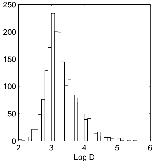
Figure 3. Distribution of the detectability parameter \log \mathcal{D} for the 1931 binaries with acceptable solutions.
