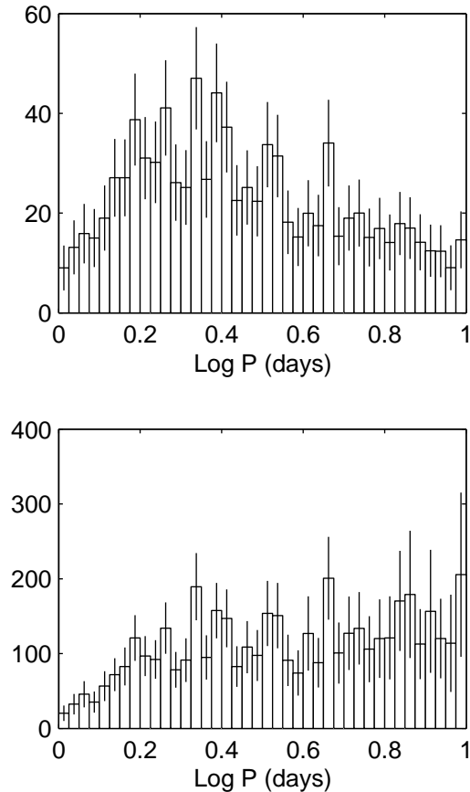
Figure 9. The period distribution of the binaries in the LMC. The top panel shows the period histogram of the trimmed sample, while the lower one shows the corrected histogram
