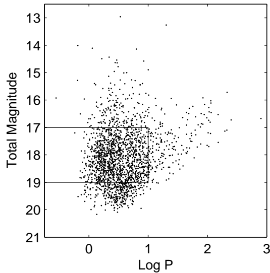
Figure 4. Total I -magnitude vs. period for 1875 binaries with accepted solutions and high enough detectability. The straight lines present the limits of the trimmed sample. Periods are in days
