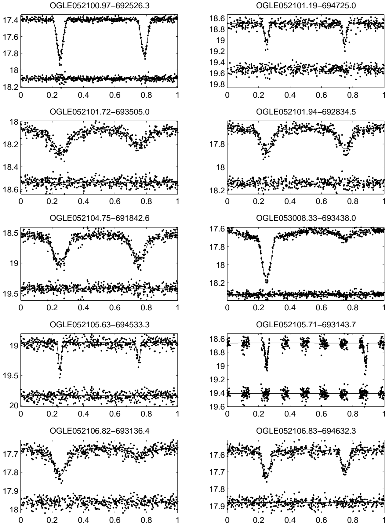
Figure 1. Ten derived lightcurves
